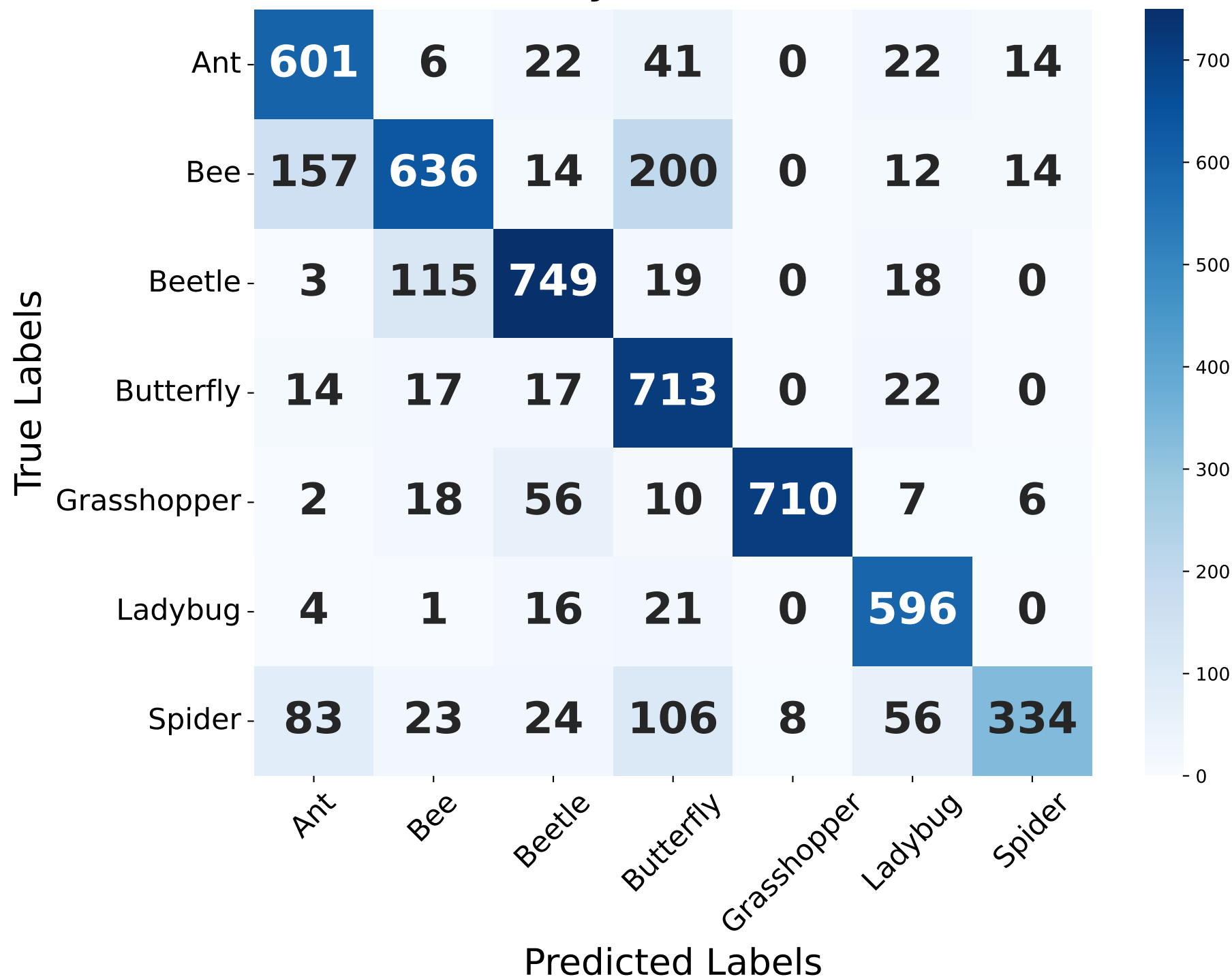
Confusion Matrix: Noisy Curated (Partial Unfreezing)
